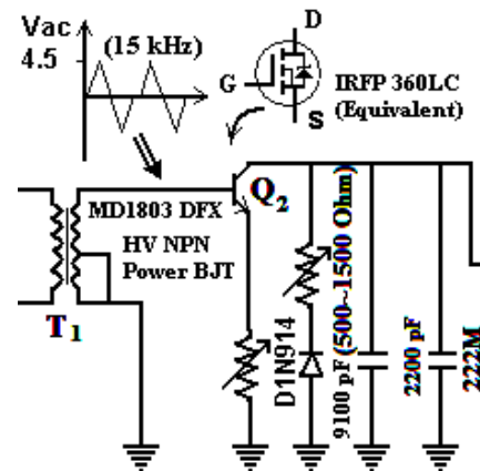
Figure: 3 Output Stage
